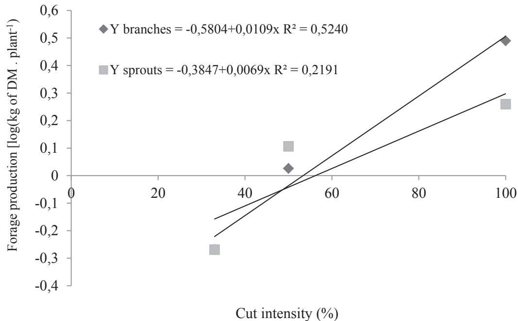
Figure 1. Regression models to estimate dry matter (DM) forage production (Y) from native Manihot glaziovii trees according to cutting intensity (X) of their fine branches ( \varnothing < 10\text{mm} ) or corresponding 1-year-old sprouts.
